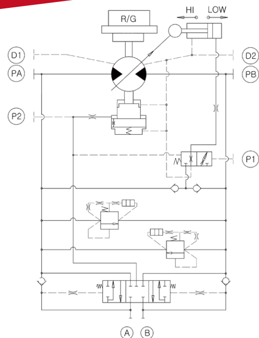
Hydraulic Circuit
